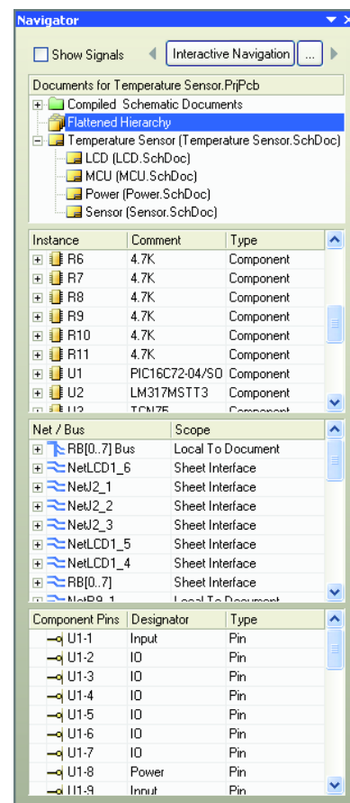
Figure 6. Use the Navigator to check the design connectivity
