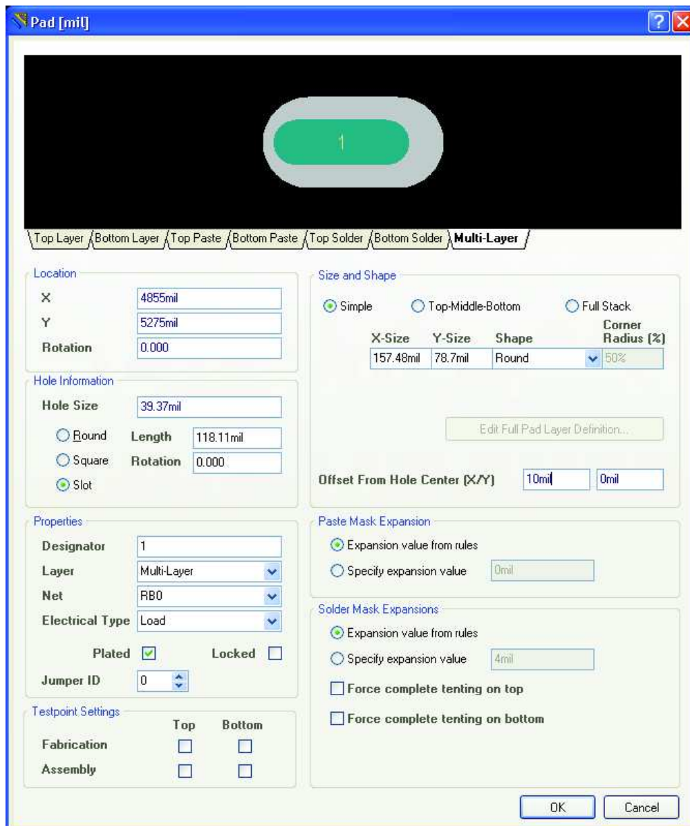
Figure 6. Pad Properties dialog
