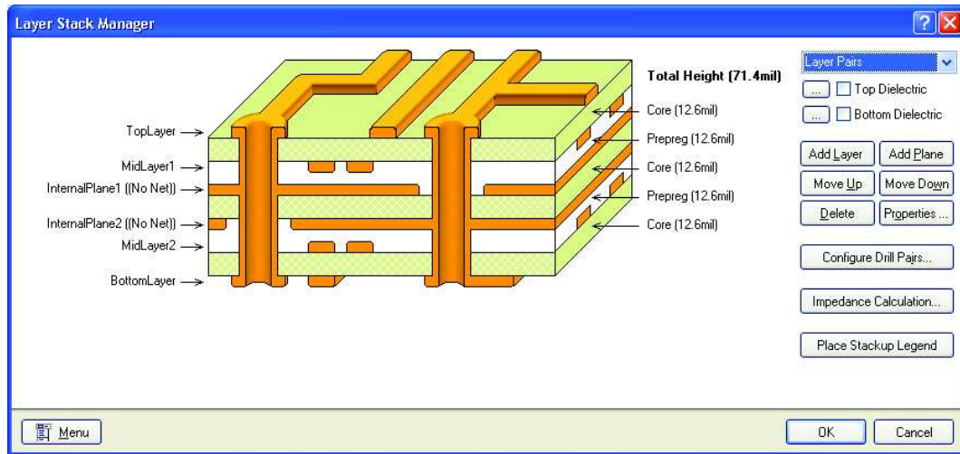
Figure 9 Layer Stack Manager dialog
