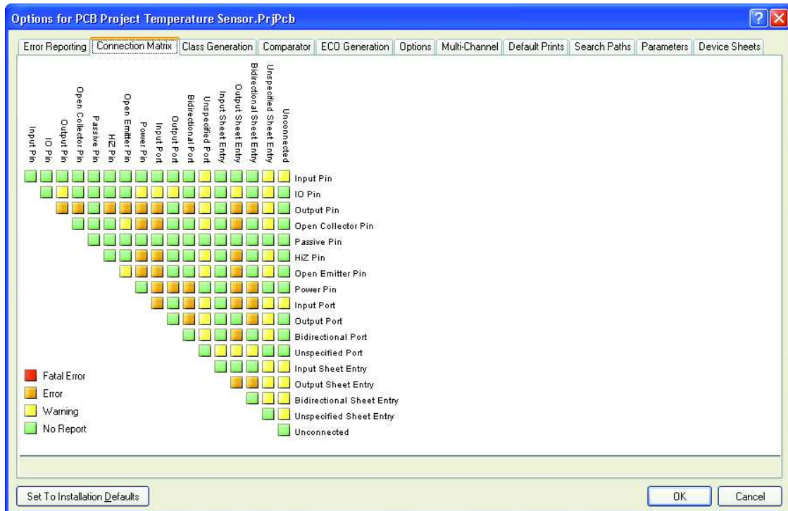
Figure 8. ERC Rule Matrix tab
