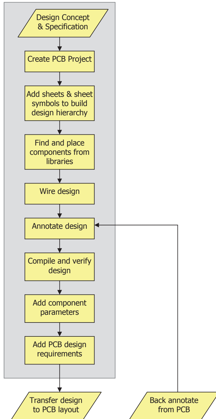
Figure 1. The Altium Designer schematic capture workflow
