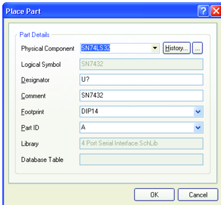
Figure 10. Place Part dialog
