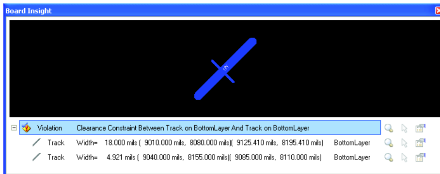
Figure 16. The board insight for Violations
