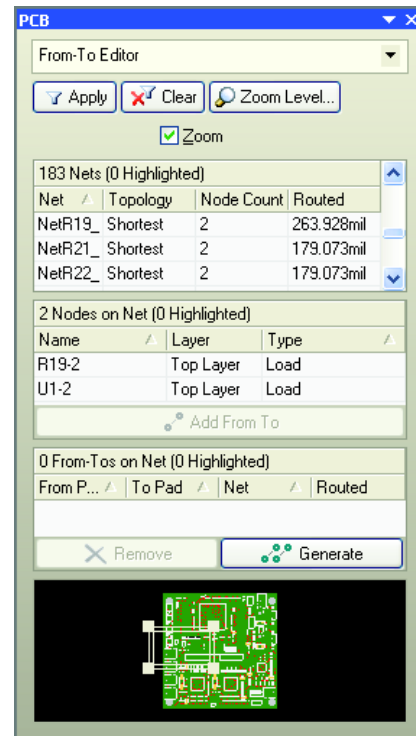
Figure 9. The From-To Editor in the PCB panel
