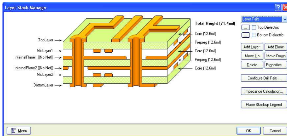
Figure 7. Define the required electrical layers in the Layer Stack Manager dialog.
