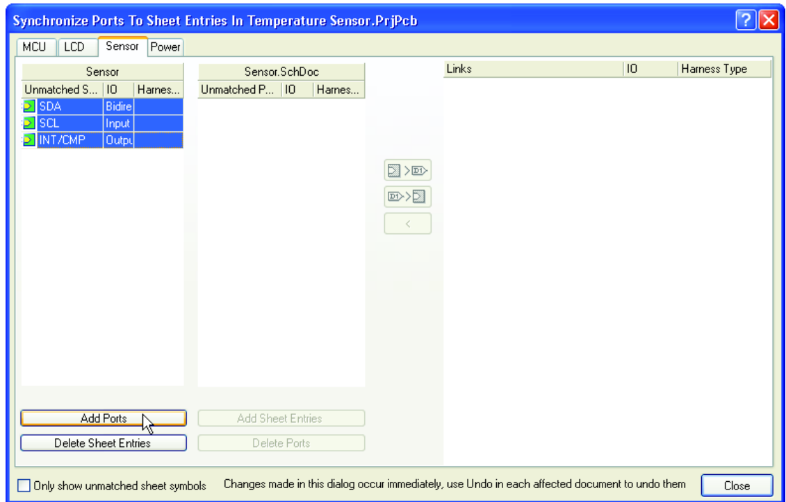
Figure 8. Problems found - missing ports on a sheet
