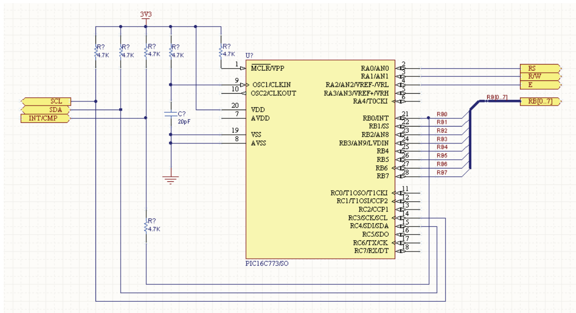
Figure 18. MCU schematic example
