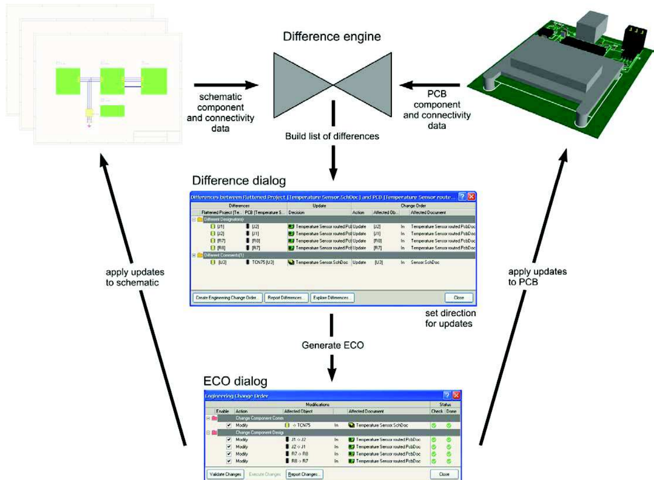
Figure 3. Design synchronization flow
