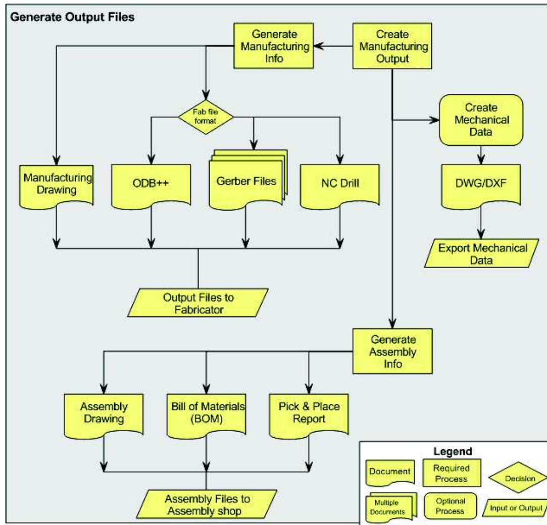
Figure 2. Work flow for generating PCB output files
