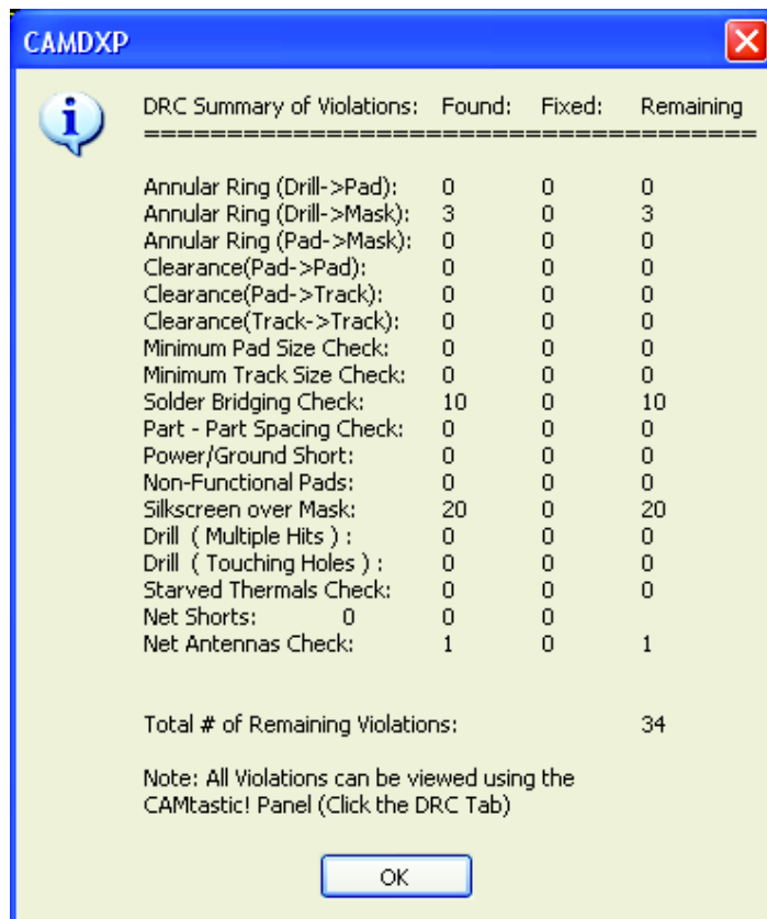
Figure 32. Results of a DRC check in Camtastic.
