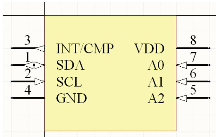
Figure 11. Microchip TCN75 serial temperature sensor
