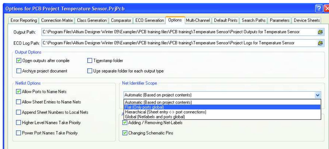
Figure 3. Net identifier scope and netlist options
