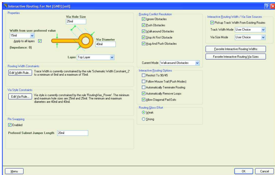
Figure 2. Interactive Routing dialog
