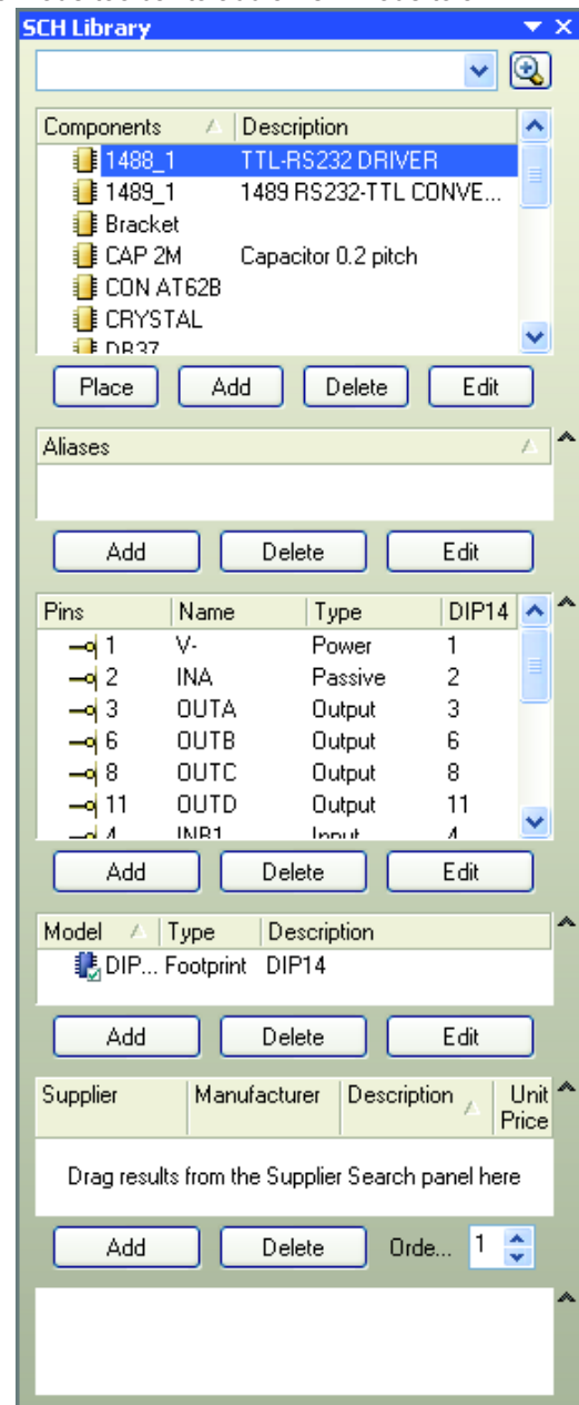
Figure 4. Schematic Library panel
