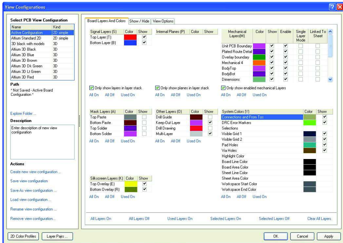
Figure 2 View Configurations dialog
