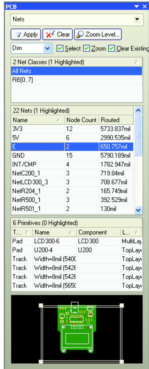
Figure 7. Browsing nets from the PCB panel
