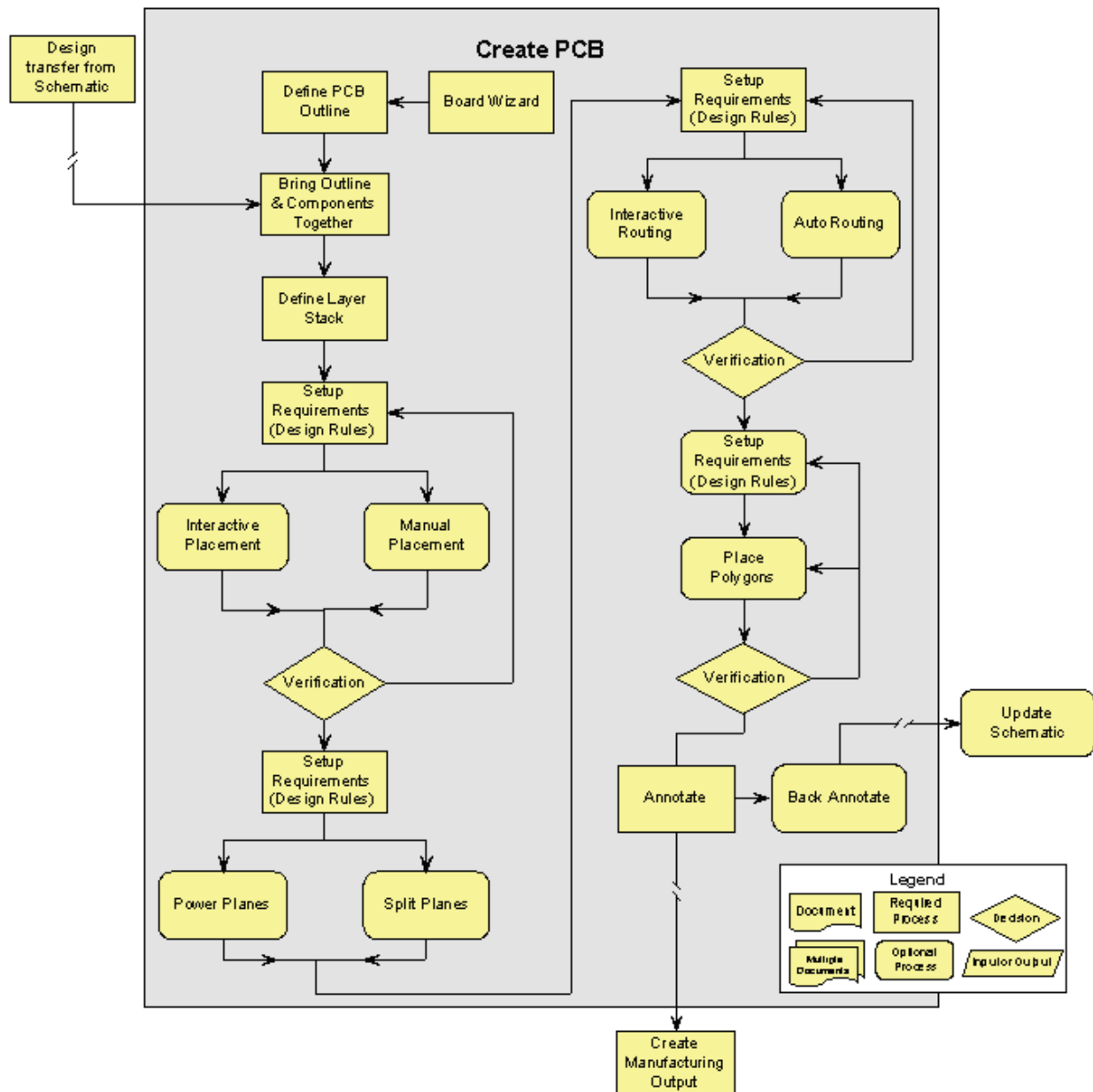
Figure 1. Overview of the PCB Design Process
