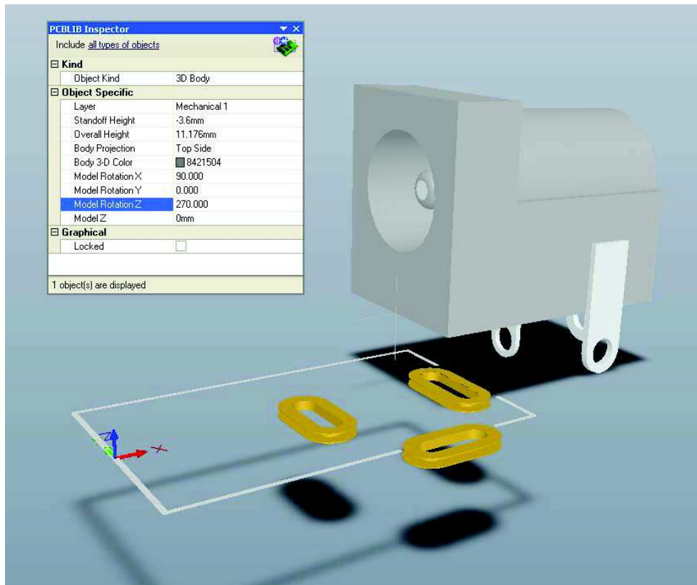
Figure 17. Use the Inspector to test different rotation values.
