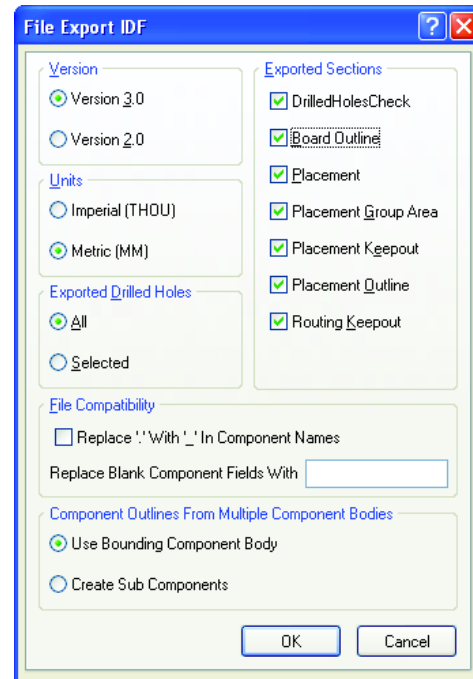
Figure 6. Export to IDF dialog
