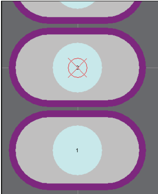
Figure 16. Pads with the solder mask displayed
