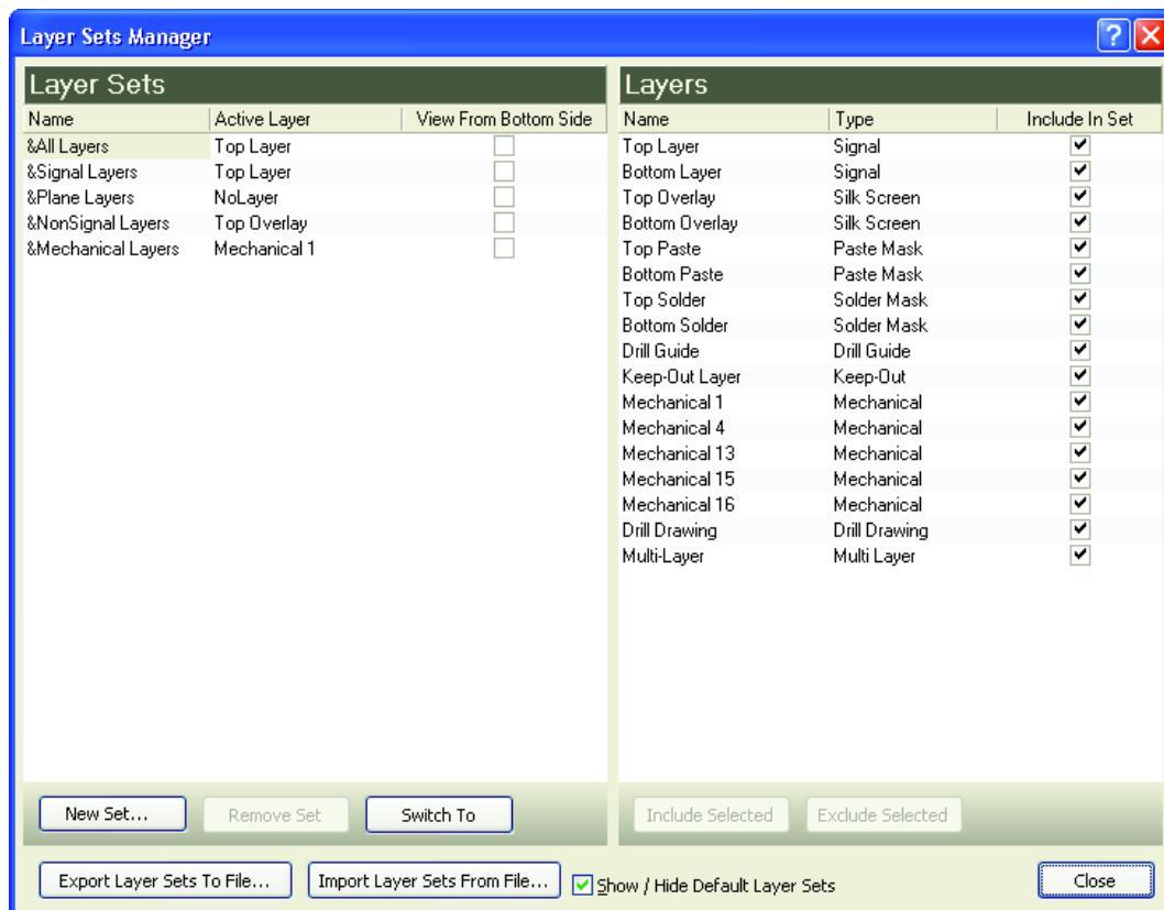
Figure 10 Defining new layer sets
