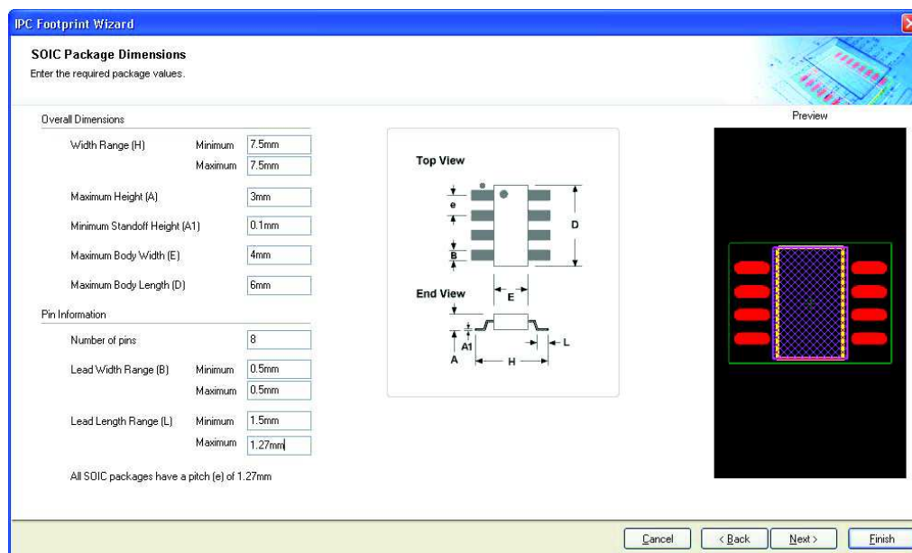
Figure 8. SOIC package dimensions
