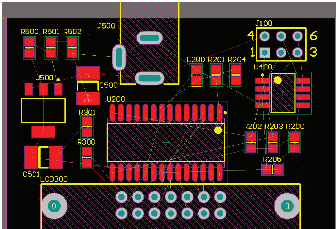
Figure 7. The placed board, ready to route.
