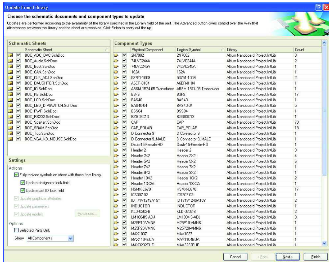
Figure 8. Update from schematic library to schematic
