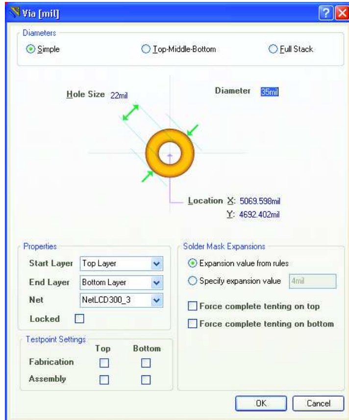
Figure 7. Via Properties dialog
