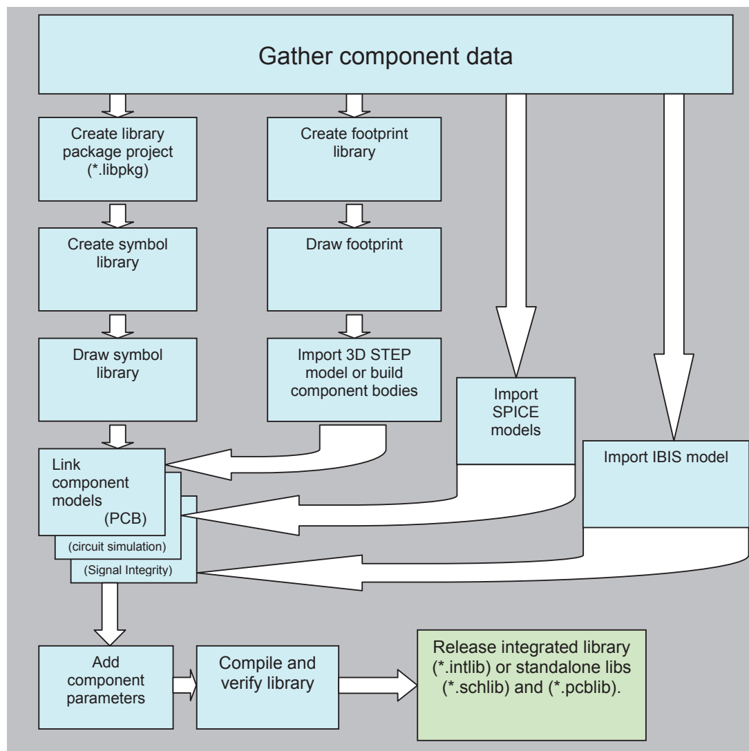
Figure 1. The Altium Designer component creation workflow.
