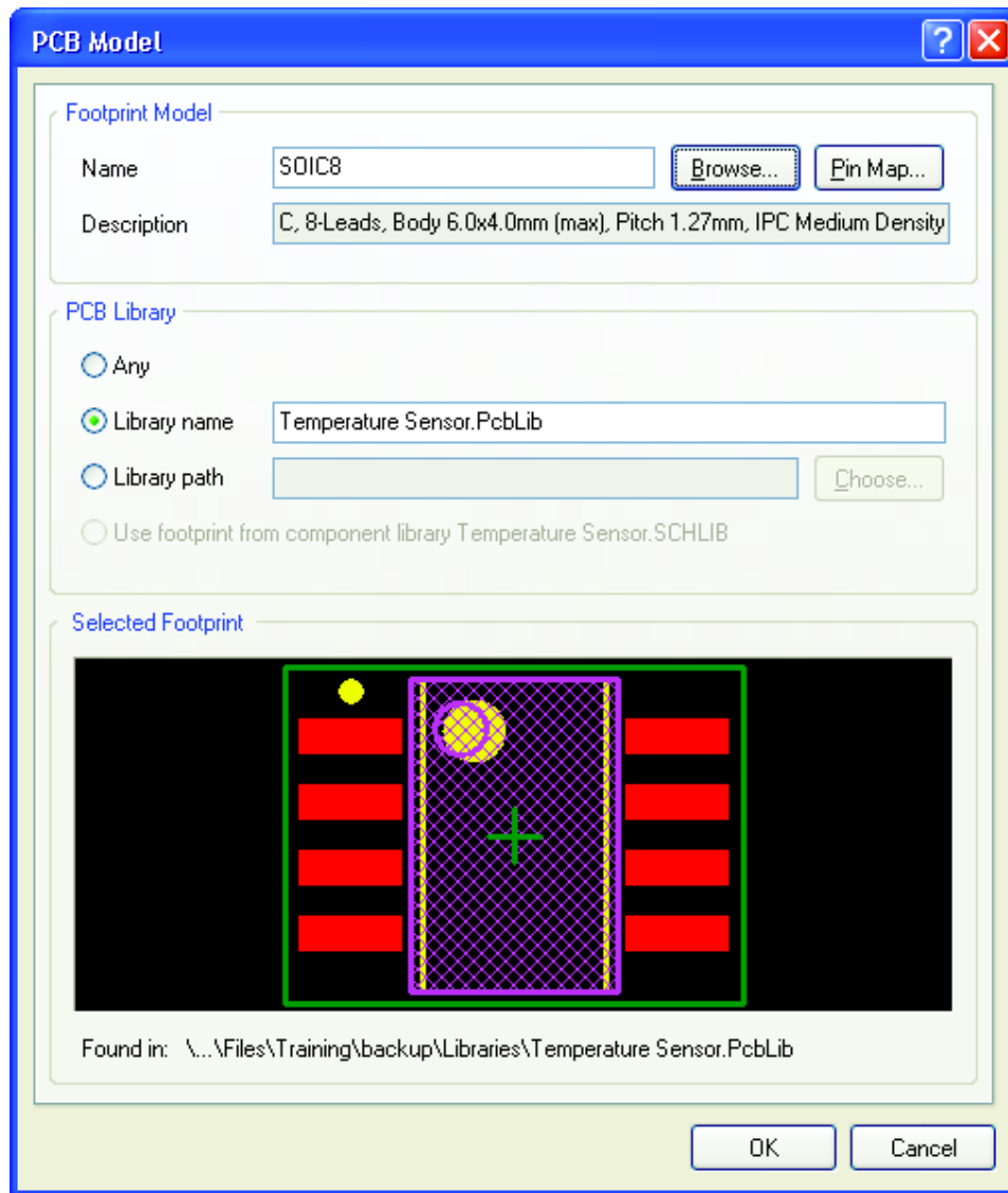
Figure 2. Adding the footprint model to the component.
