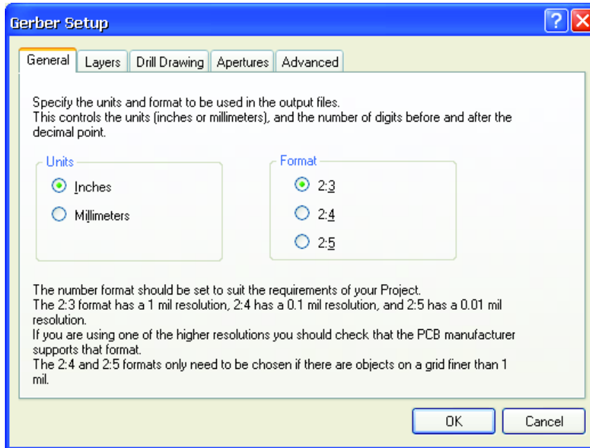
Figure 15. Gerber Setup dialog
