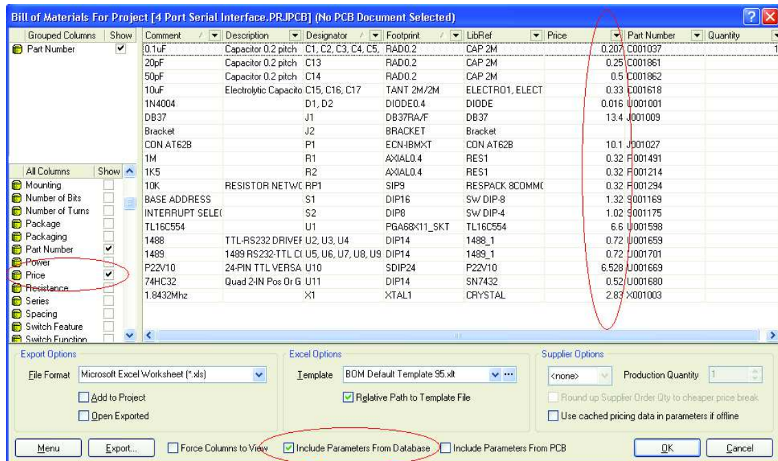
Figure 6. Include additional component information that exists only in an external database
