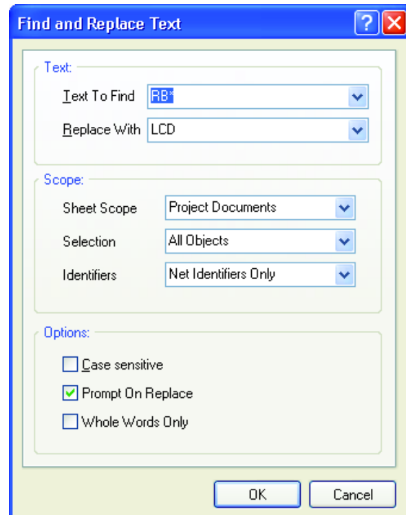
Figure 1. Performing a partial string substitution
