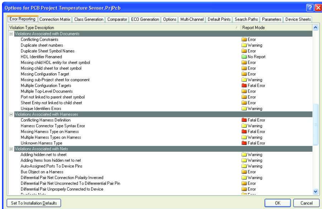
Figure 7. Setup for Error Reporting
